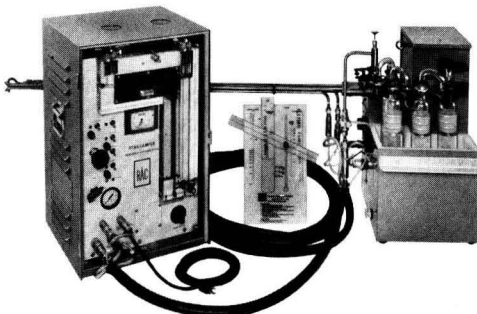
RAC Train Staksampl™ System (EPA Method) Circle No. 39 on Readers' Service Card
